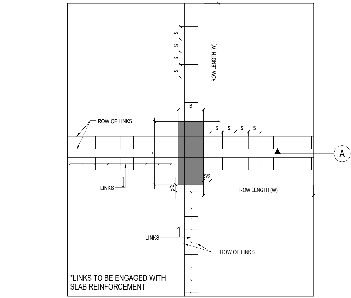
INTERNAL COLUMNS
