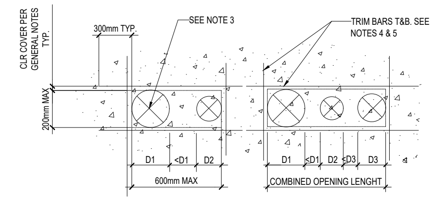
OPENINGS UP TO 600mm
