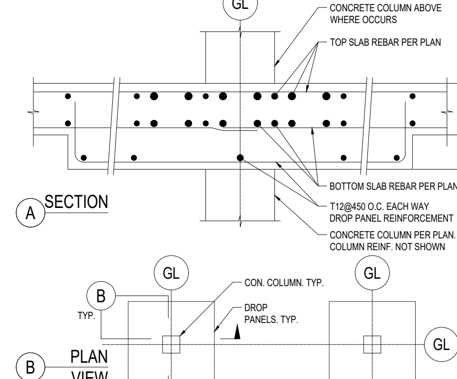
ISOLATED DROP PANEL
