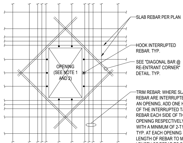
OPENINGS WITH AT LEAST ONE SIDE GREATER THAN 600mm
