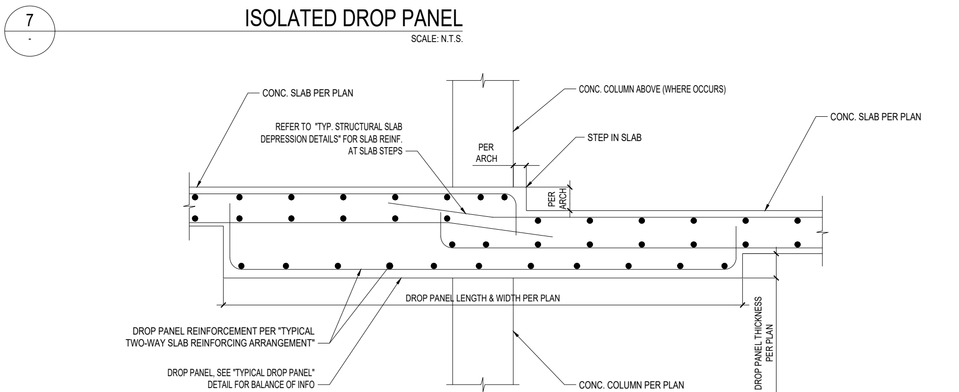
ISOLATED DROP PANEL
