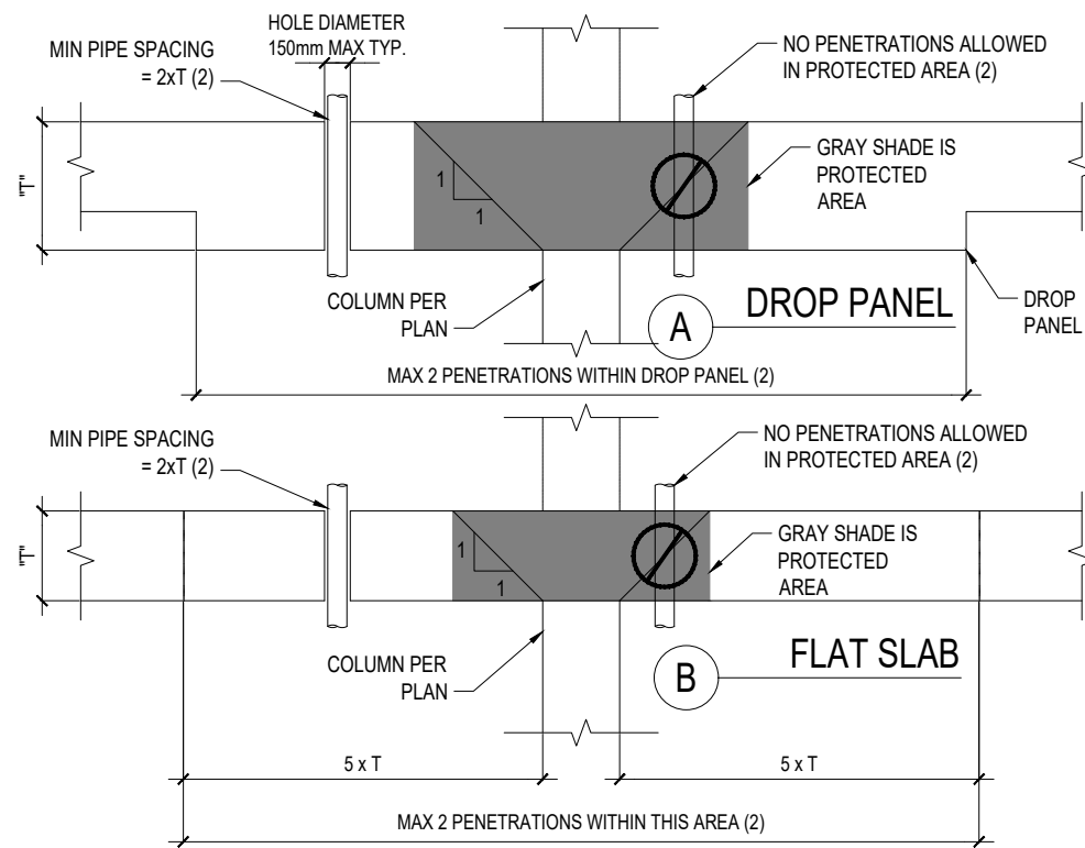
SLAB PENETRATIONS CLOSE TO COLUMNS
