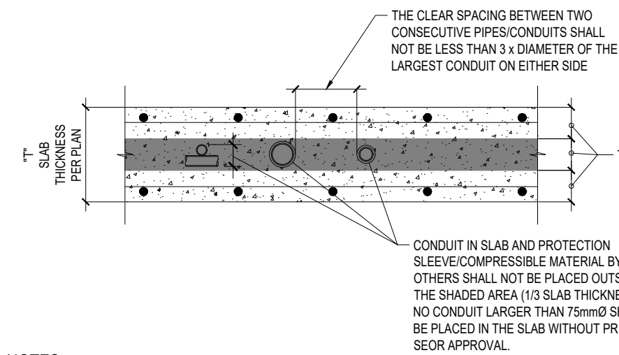
SLAB OPENINGS AND PENETRATIONS
