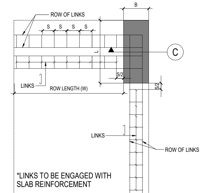
CORNER COLUMNS
